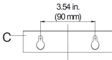
Mounting Template
