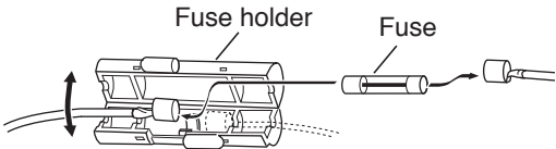
Fuse holder (K, M4 types)
