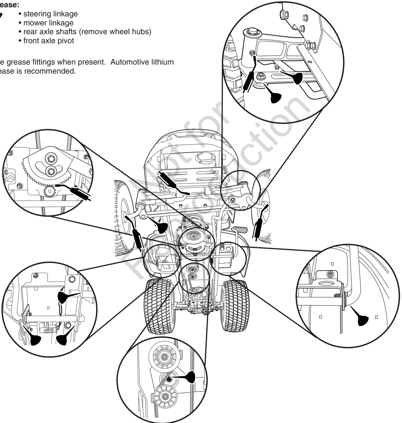
Figure 14. Lubricate Tractor
