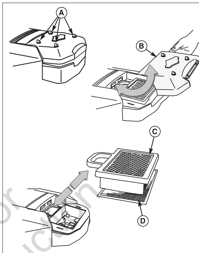
Figure 26. Air Filter Assembly - Briggs & Stratton Twin Cylinder Models
