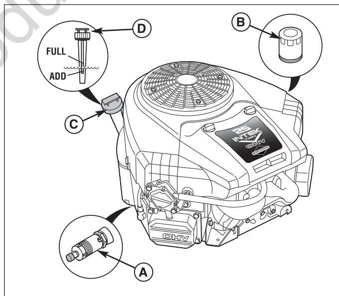
Figure 23. Briggs & Stratton Twin Cylinder Models
