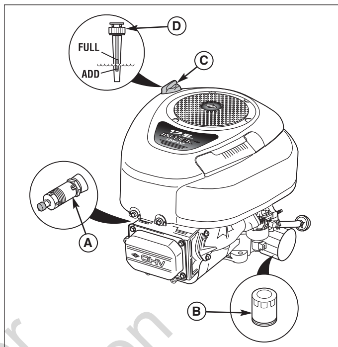
Figure 22. Briggs & Stratton Single Cylinder Models
