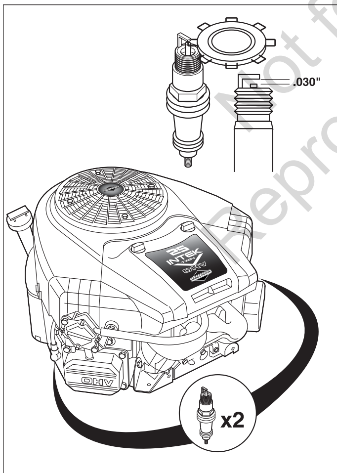
Figure 31. Spark Plug Gapping
