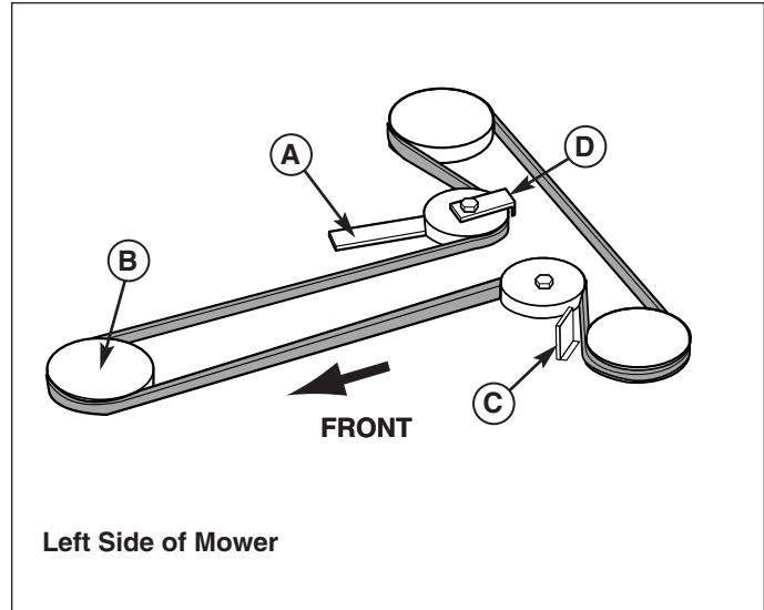
Figure 41. Typical Mower Belt Routing Two Blade Decks
