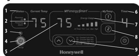
Model HZ-980 User Interface Controls:
