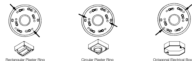
FIGURE 2. SELECT CORRECT MOUNTING HOLES ON TRIM RING
