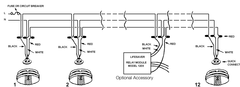
FIGURE 1 INTERCONNECT WIRING DIAGRAM
