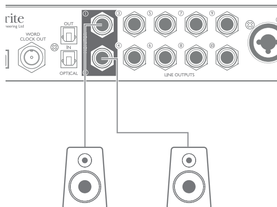
Active Speakers
