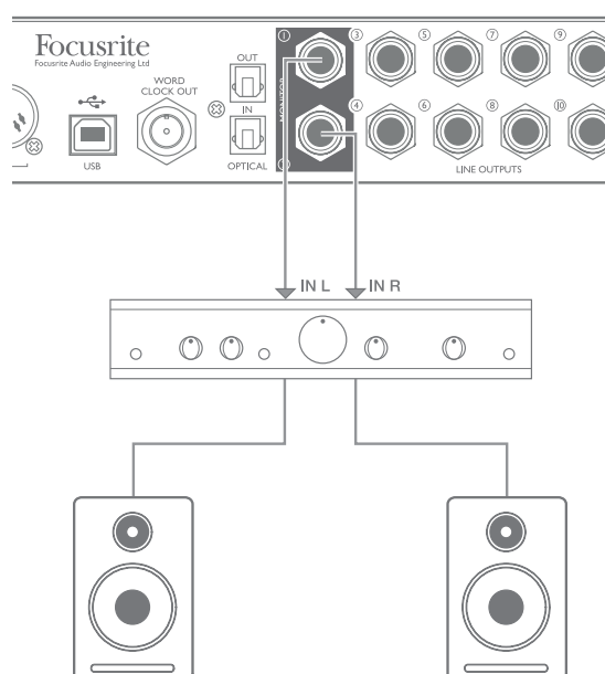
Passive Speakers
