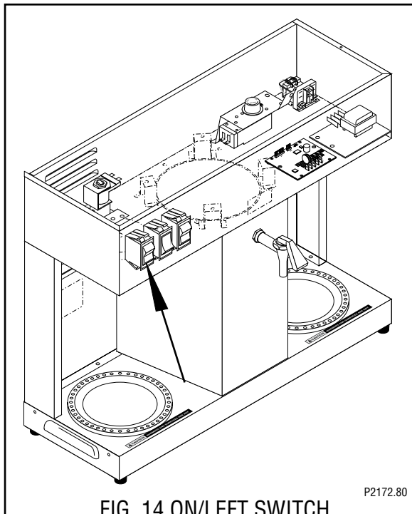
FIG. 14 ON/LEFT SWITCH
