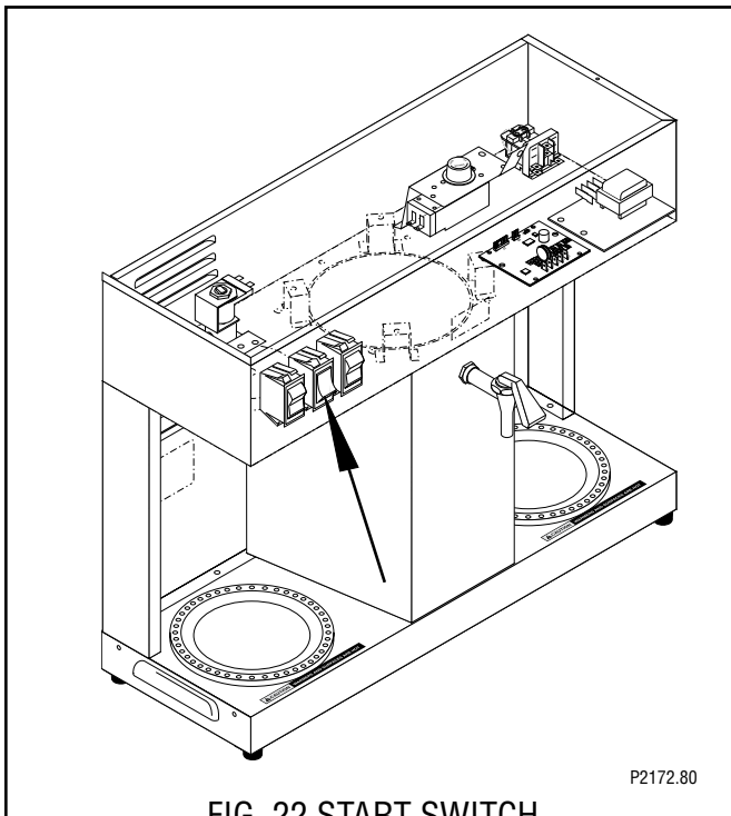
FIG. 22 START SWITCH
