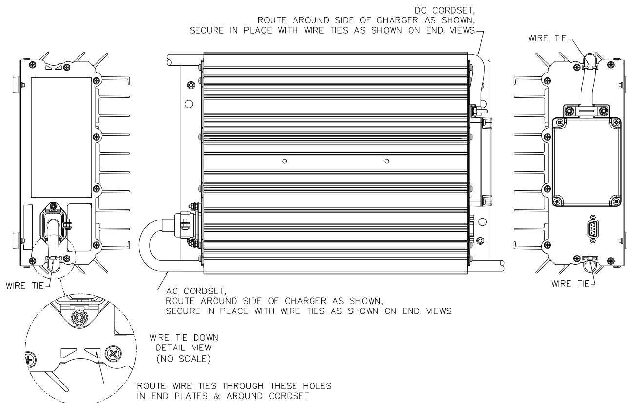
Figure 2-3: AC & DC Cordset Routing
