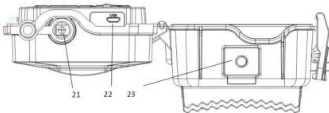
Fig. 3: Bottom view
