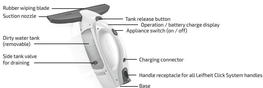
Figure 2: Window cleaner operating controls
