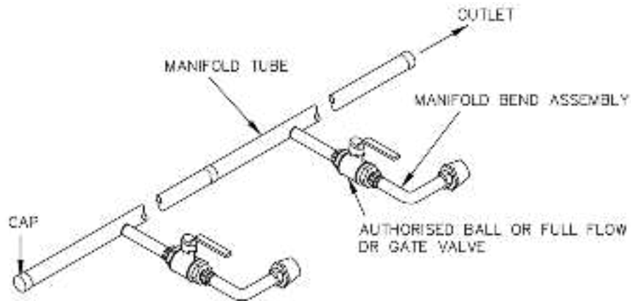
Hot Manifold Assembly
