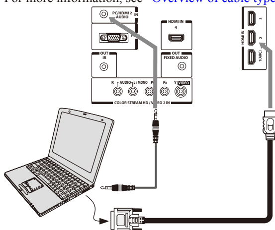
(Sample Illustration) L9300U Series—Connecting to an HDMI™ terminal
