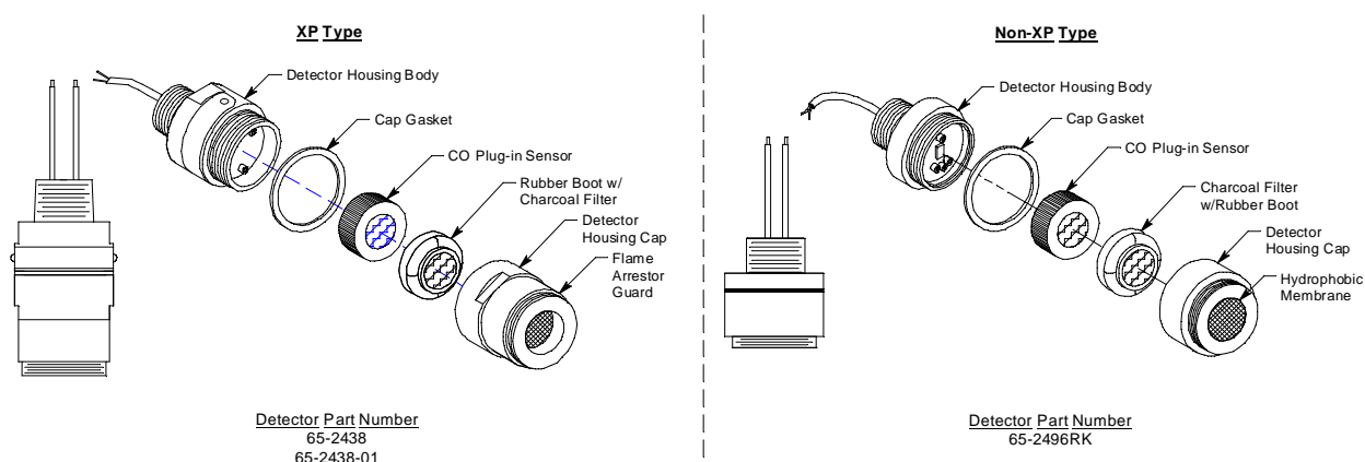
Figure 6: CO Detectors
