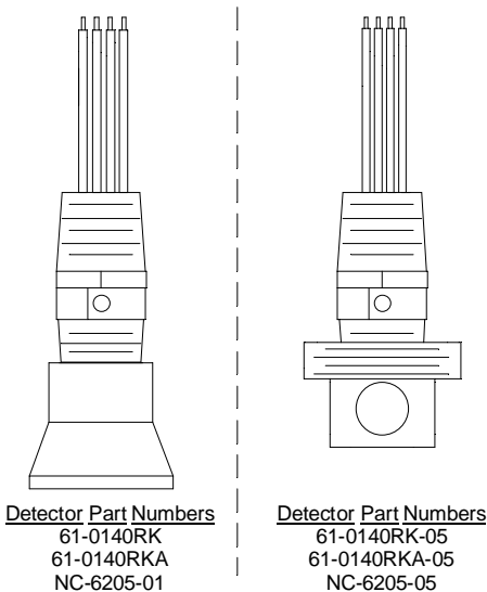
Figure 2: Catalytic Sensors
