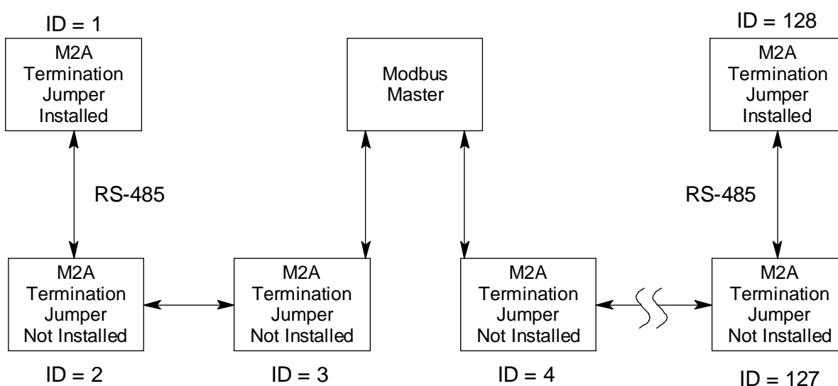
Figure 34: Multiple M2As in a Daisy Chain Configuration
