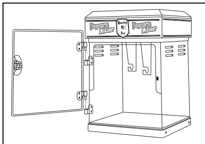
FIGURE 1 Place door on hinges.
