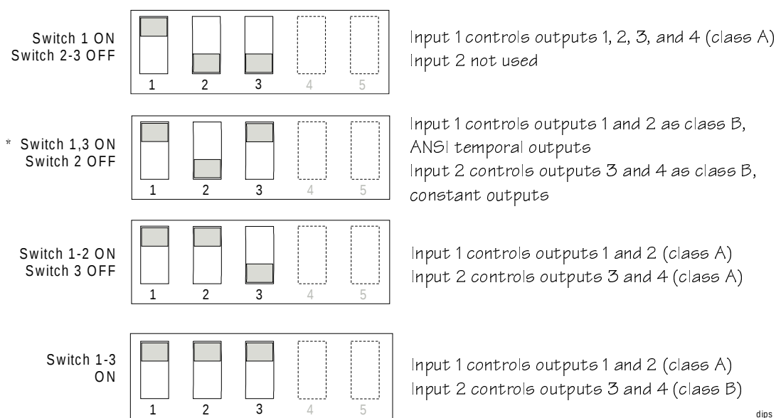
Figure 4-7. Setting DIP Switches 1-3
