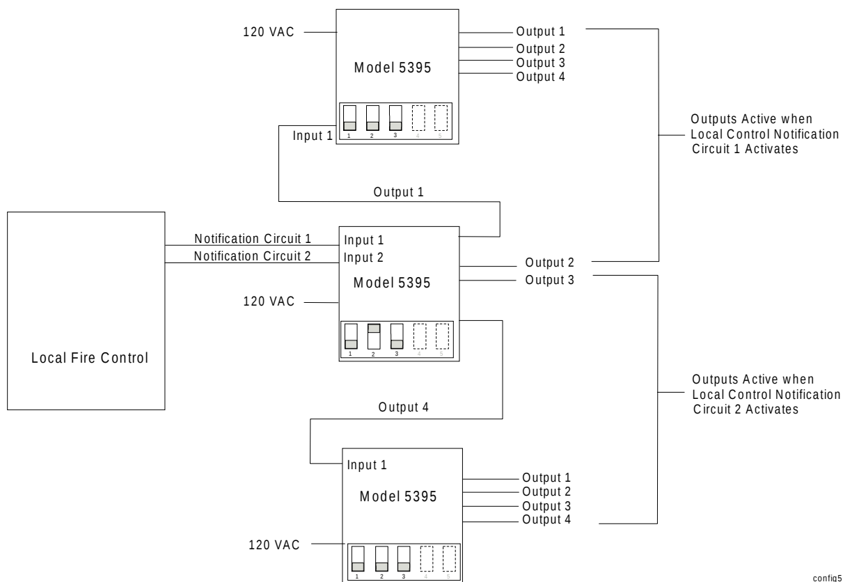
Figure 6-5. Each Control Signal Circuit Activates Five Output Circuits
