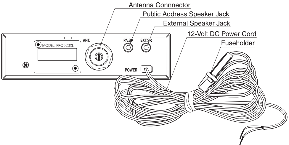
BACK VIEW
