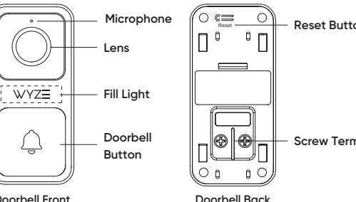
Doorbell Front
