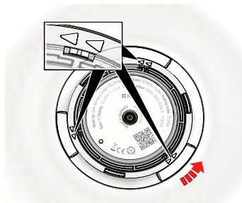
Filter replacement back cover opening direction.
