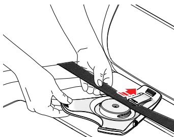
Step 2: Slide the car mount under the belt into the belt hook.
