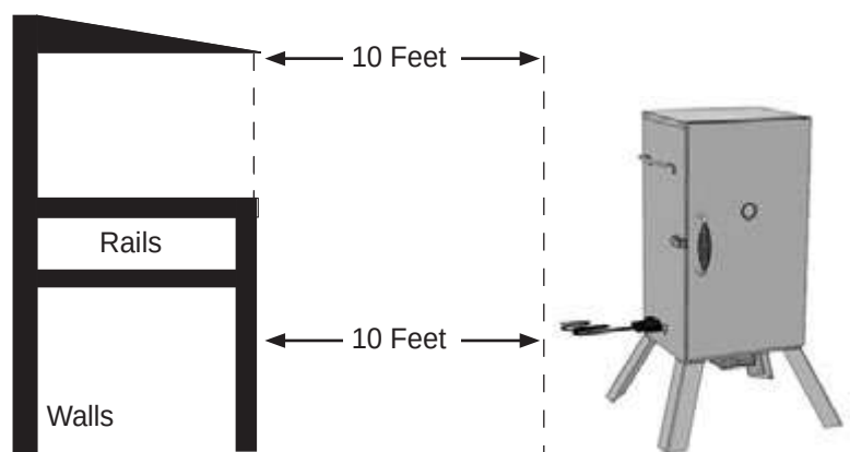
Overhead Construction
